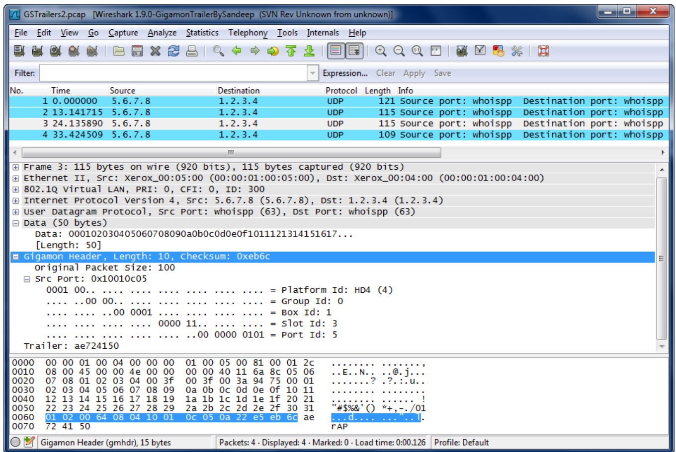
Figure 166 Wireshark Decode of GigaSMART Trailer
