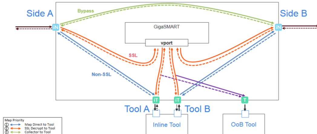
Figure 104 Packet Flow for Inline SSL Decryption
