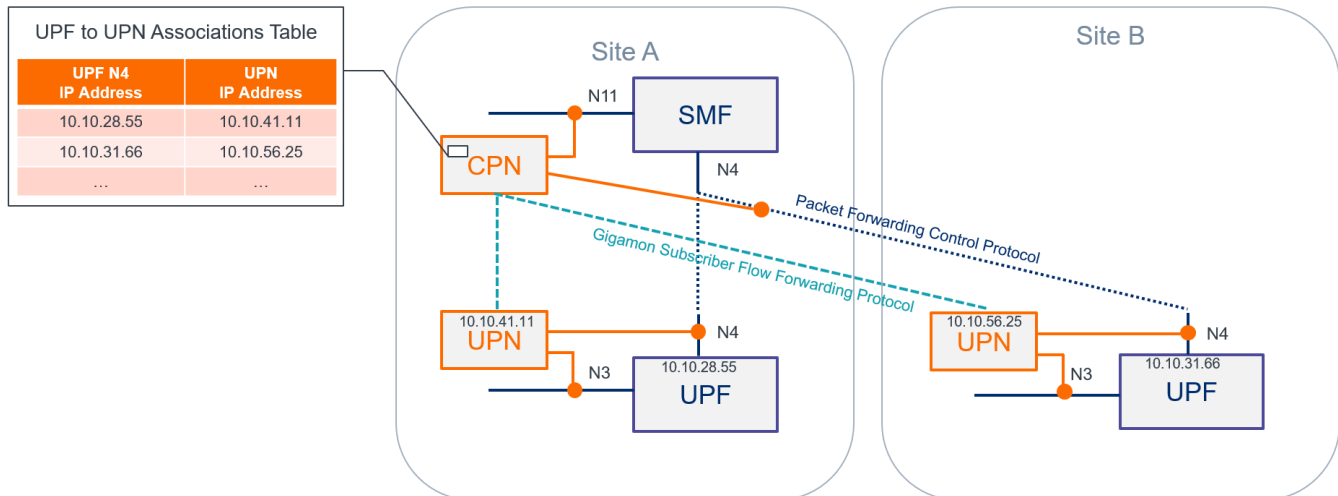
Figure 38 Dynamic CPN-to-UPN Mapping for 5G CUPS
