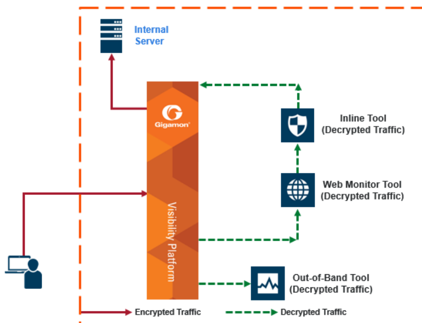
Figure 101 Inbound Deployment of Inline SSL Decryption
