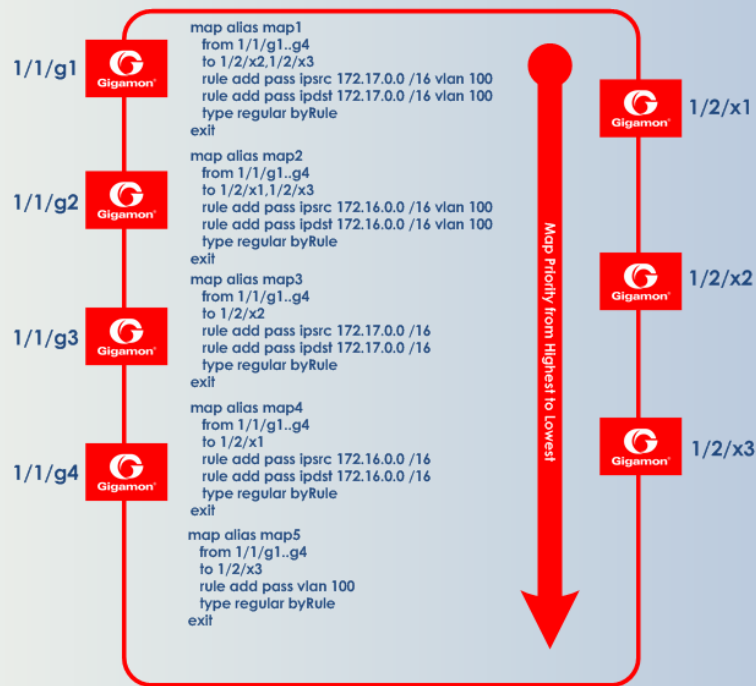
Figure 11 Sending Subnets and VLANs to Different Ports
