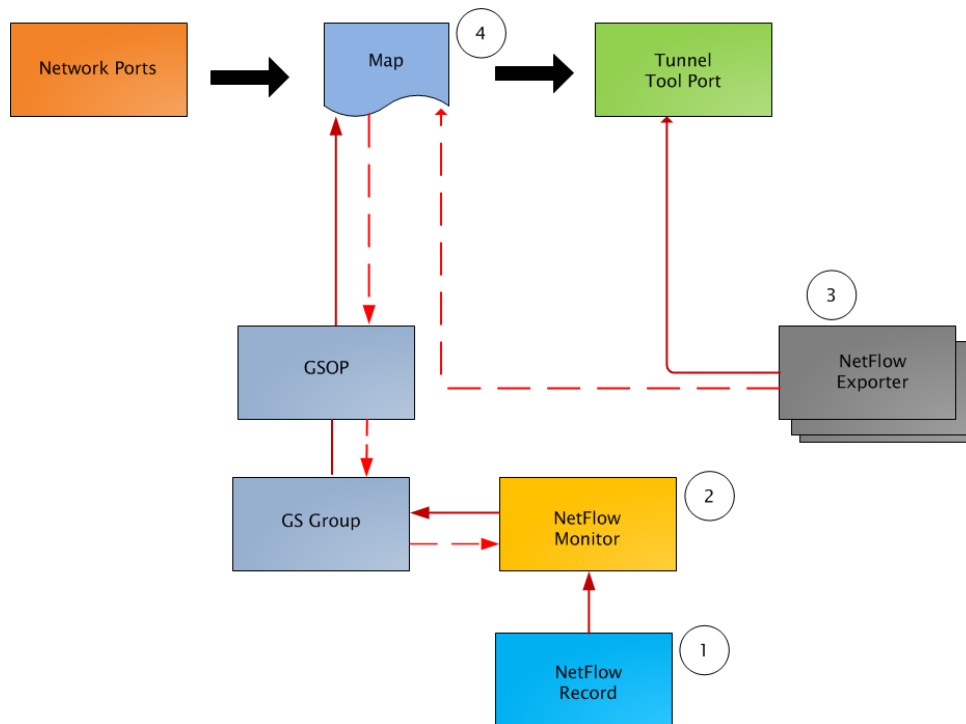
Figure 80 NetFlow Generation Components
