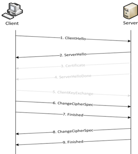
Figure 124 Resumed SSL Handshake
