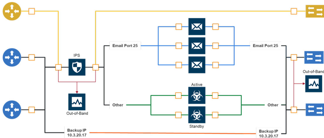
Figure 16 Flexible Inline Arrangements Scenario
