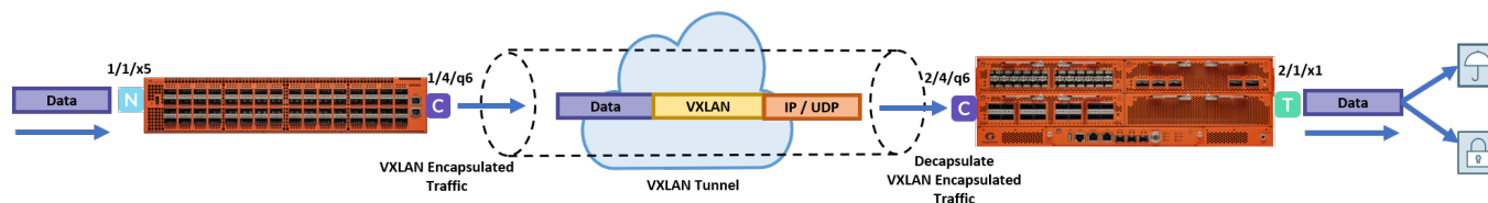
Figure 31 VXLAN Tunnel Encapsulation and Decapsulation
