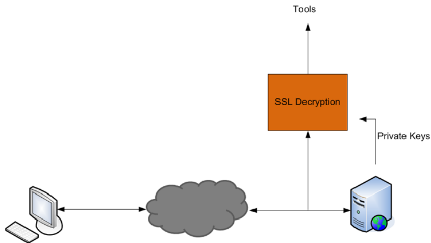
Figure 125 Inbound (Server Side)
