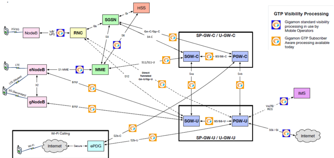
Figure 30 3GPP CUPS Network topology
