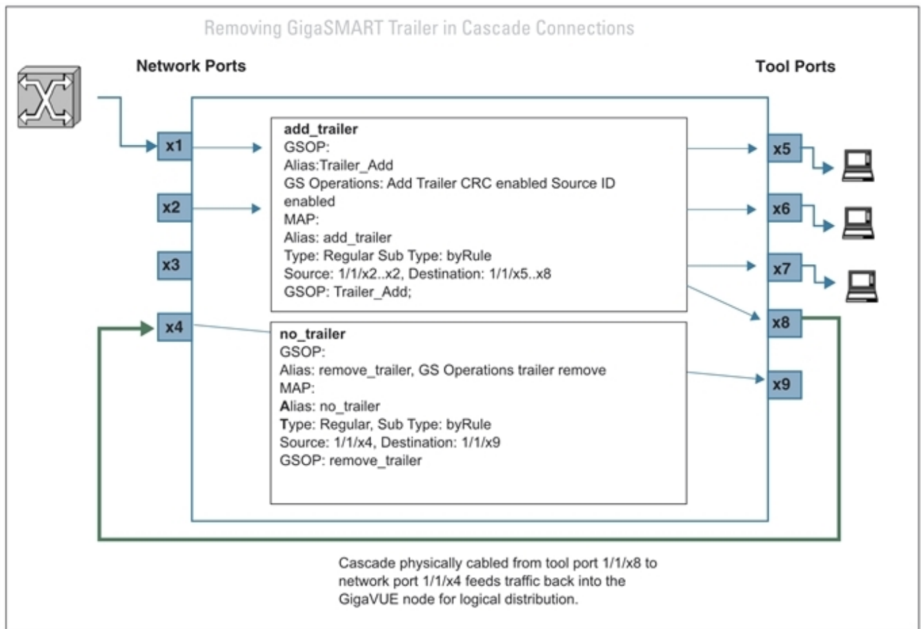
Figure 164 Removing the GigaSMART Trailer from a Cascade Connection
