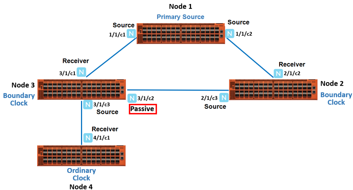
Figure 25 PTP Deployment
