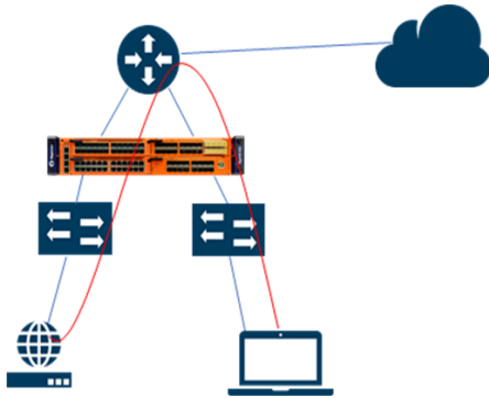
Figure 97 Inline SSL Inline Network Group Configuration
