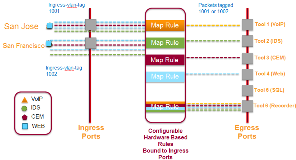
Figure 12 Using Ingress Port VLAN Tagging
