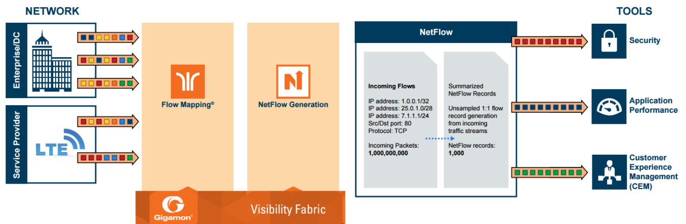
Figure 79 NetFlow Generation Gigamon Solution
