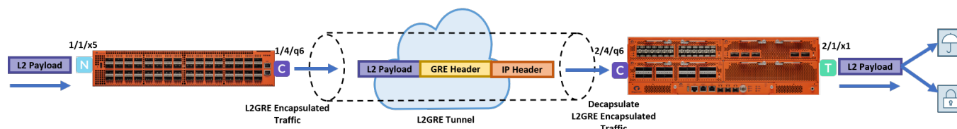
Figure 30 L2GRE Tunnel Encapsulation and Decapsulation
