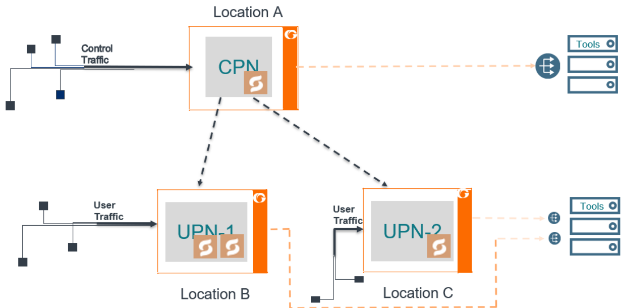
Figure 31 Topology diagram of CPN and UPN Connections
