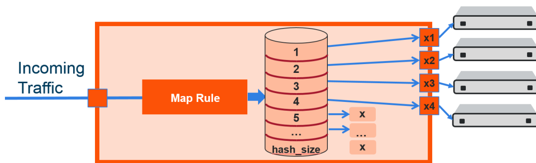
Figure 19 Controlled GigaStream Overview
