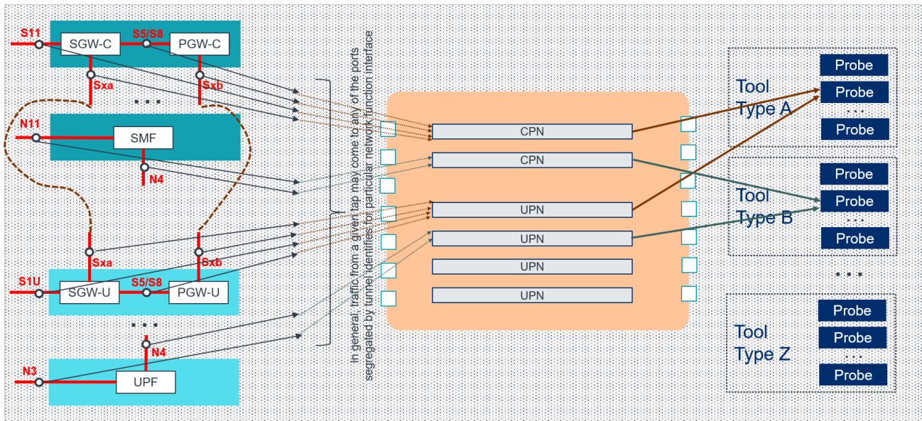
Figure 37 Traffic Correlation for LTE and 5G CUPS
