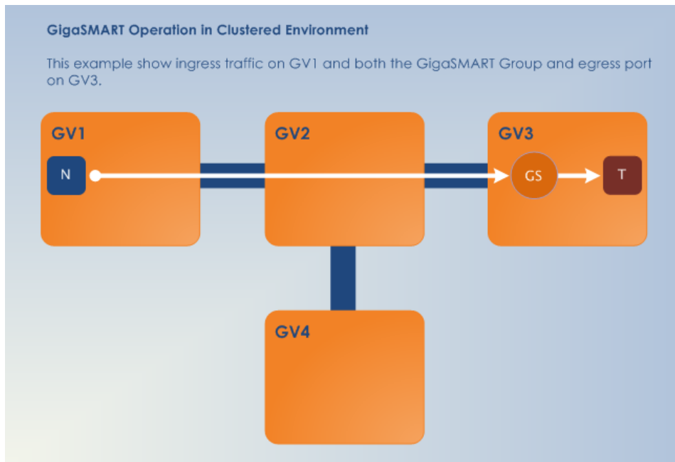
Figure 156 GigaSMART Operations in Clusters
