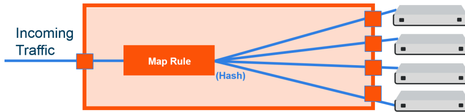
Figure 16 Regular GigaStream Overview
