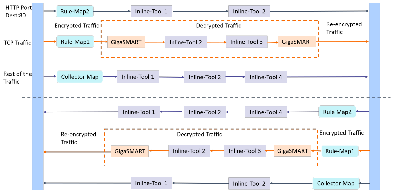
Figure 20 Flexible Inline Decryption Solution
