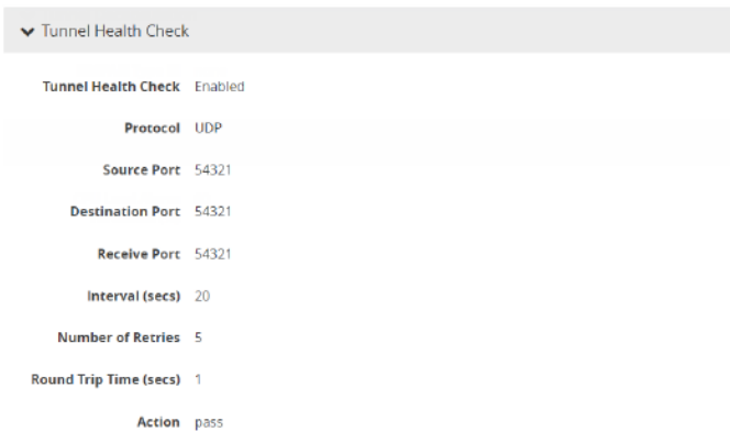
Figure 150 Configure UDP Health Check Parameters
