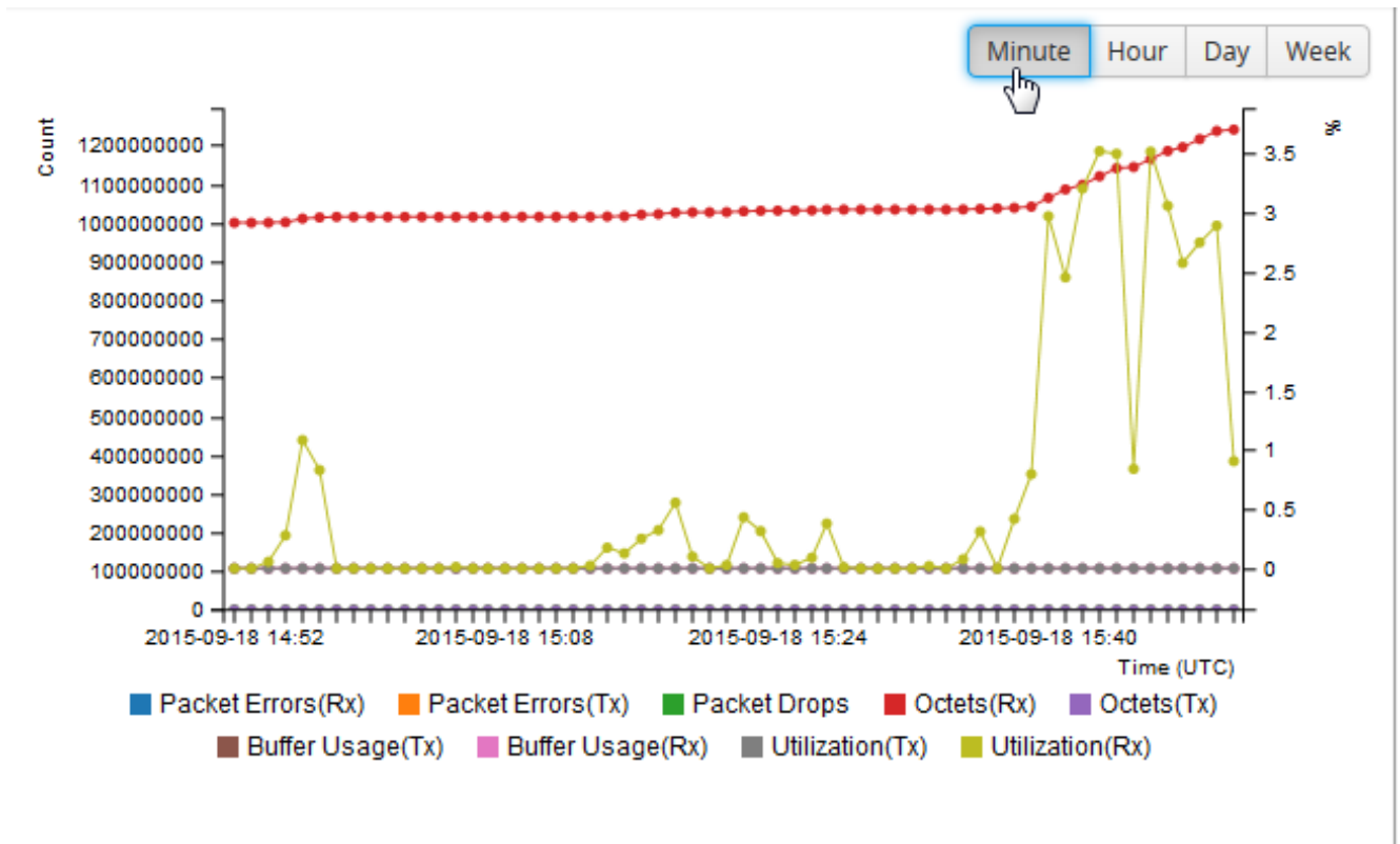
Figure 27 Numerical Values for the Data Points Measured by Hour
