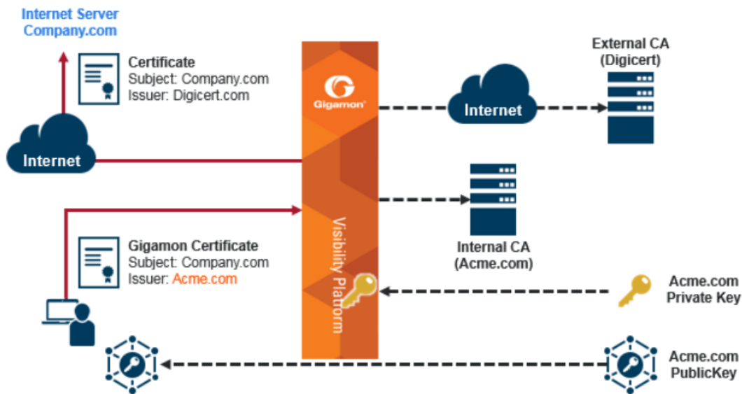
Figure 102 Outbound Deployment of Inline SSL Decryption
