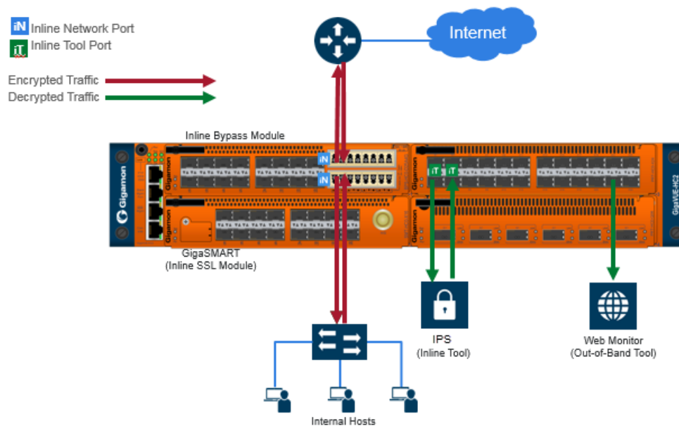
Figure 103 GigaVUE Modules: GigaSMART and Inline Bypass
